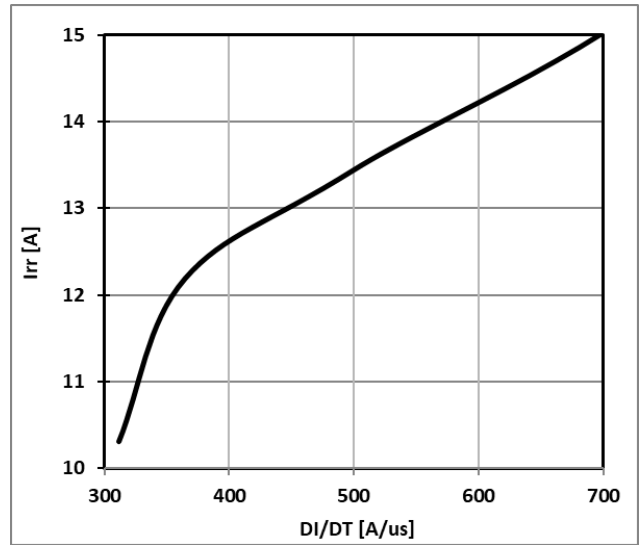
Figure 14: Typical Diode IRR VS. DI/DT, TC=25°C VCC=600V, VGE=15V, IF=15A
