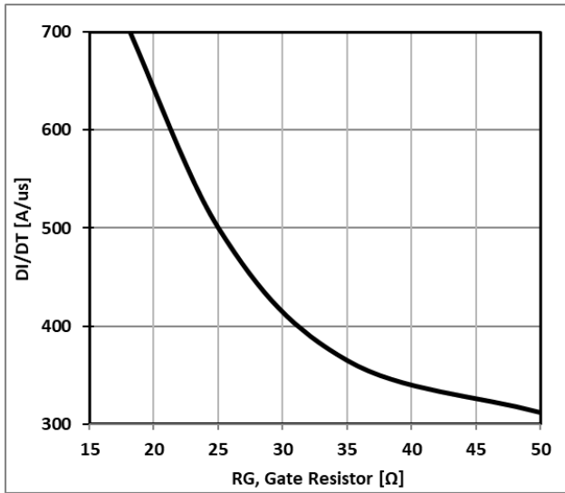
Figure 13: Typical Diode DI/DT VS. RG, TC=25°C VCC=600V, VGE=15V, IF=15A
