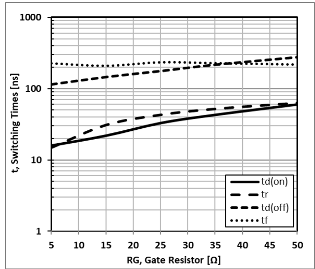
Figure 10: Typical Switching Time VS. RG, TC=25°C, L=200uH, VCE=600V, VGE=15V, IC=15A
