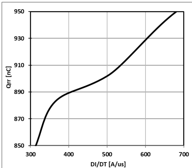
Figure 15: Typical Diode Qrr VS. DI/DT, TC=25°C VCC=600V, VGE=15V, IF=15A
