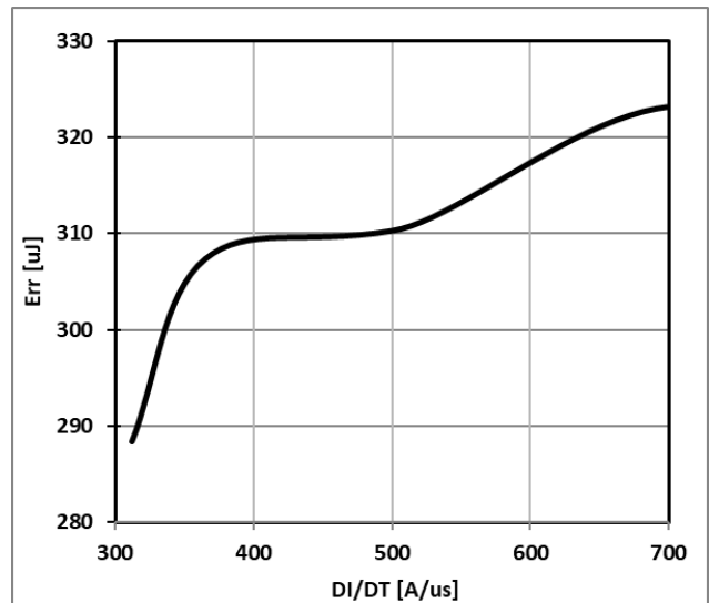
Figure 16: Typical Diode Err VS. DI/DT, TC=25°C VCC=600V, VGE=15V, IF=15A
