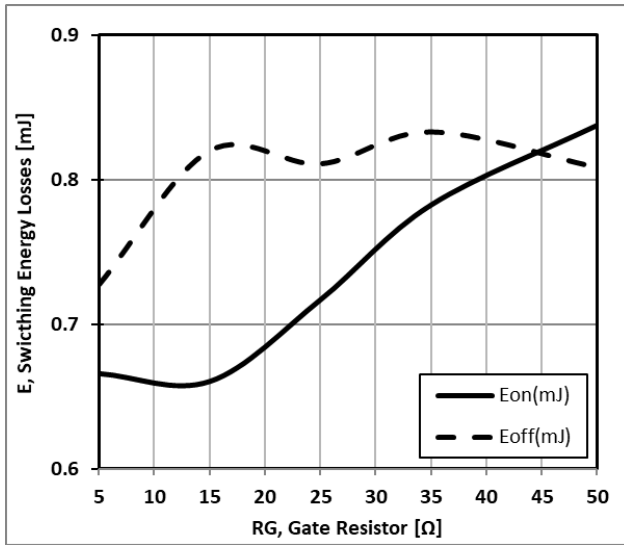
Figure 9: Typical Energy Loss VS. RG, TC=25°C, L=200uH, VCE=600V, VGE=15V, IC=15A
