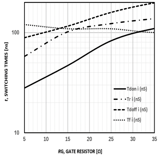
Figure10: Typical switching time VS. Rg,TC=25°C, VCE=600V, VGE=15V ,IC=25A
