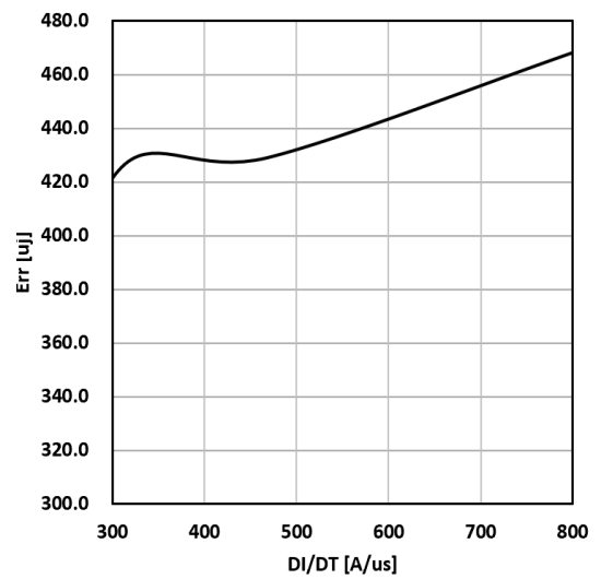
Figure 16. Typical diode Err vs di/dt Tc=25°C VCC=600V VGE=15V IF=25A
