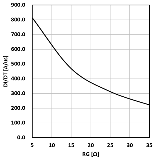
Figure 13. Typical diode di/dt vs rg Tc=25°C VCE=600V VGE=15V IF=25A
