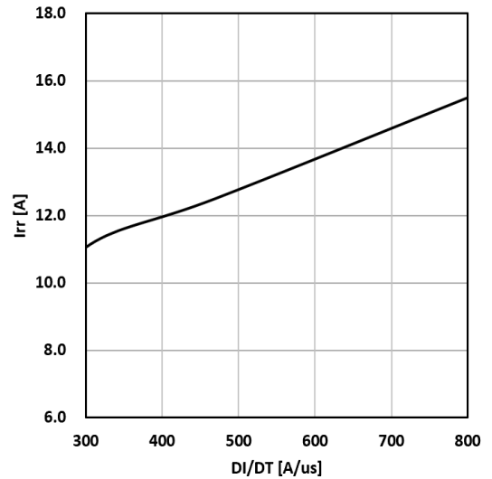
Figure 14. Typical diode Irr vs di/dt Tc=25°C VCE=600V VGE=15V IF=25A
