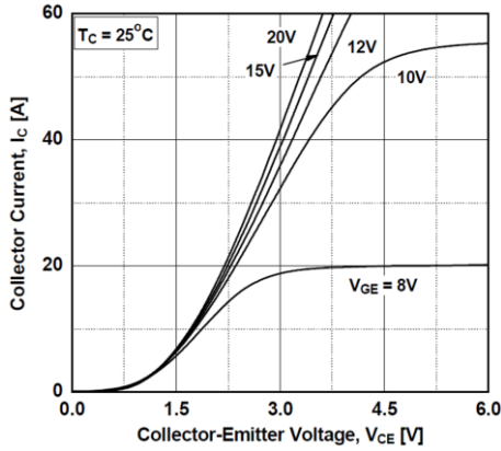
Fig 1. Output characteristics
